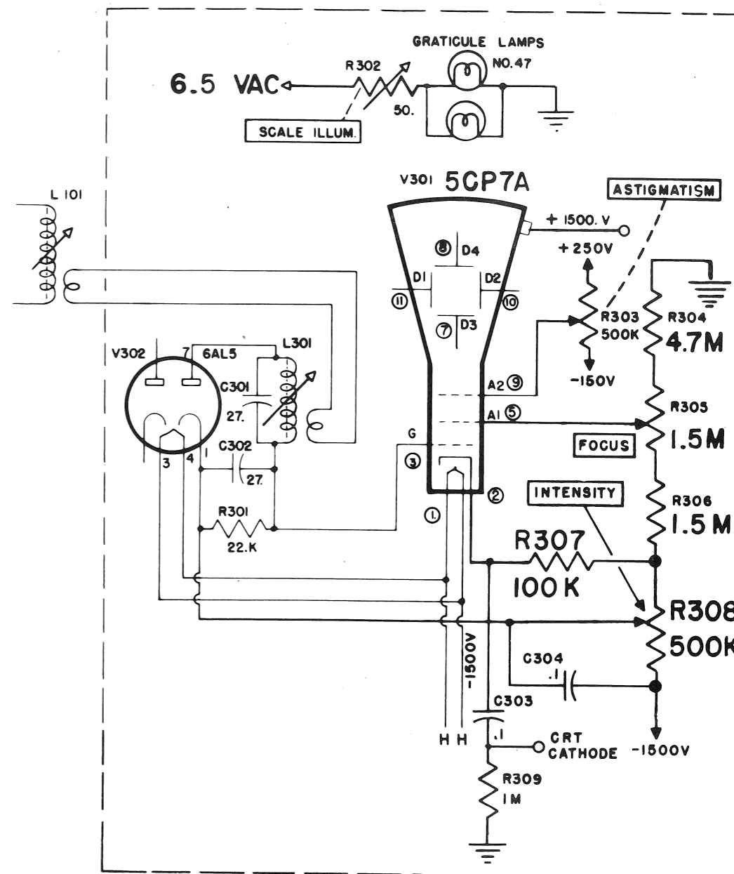
CRT CIRCUIT FOR S/N 101-2146 ONLY. SEE SWEEP DIAGRAM FOR S/N 2147 UP.
