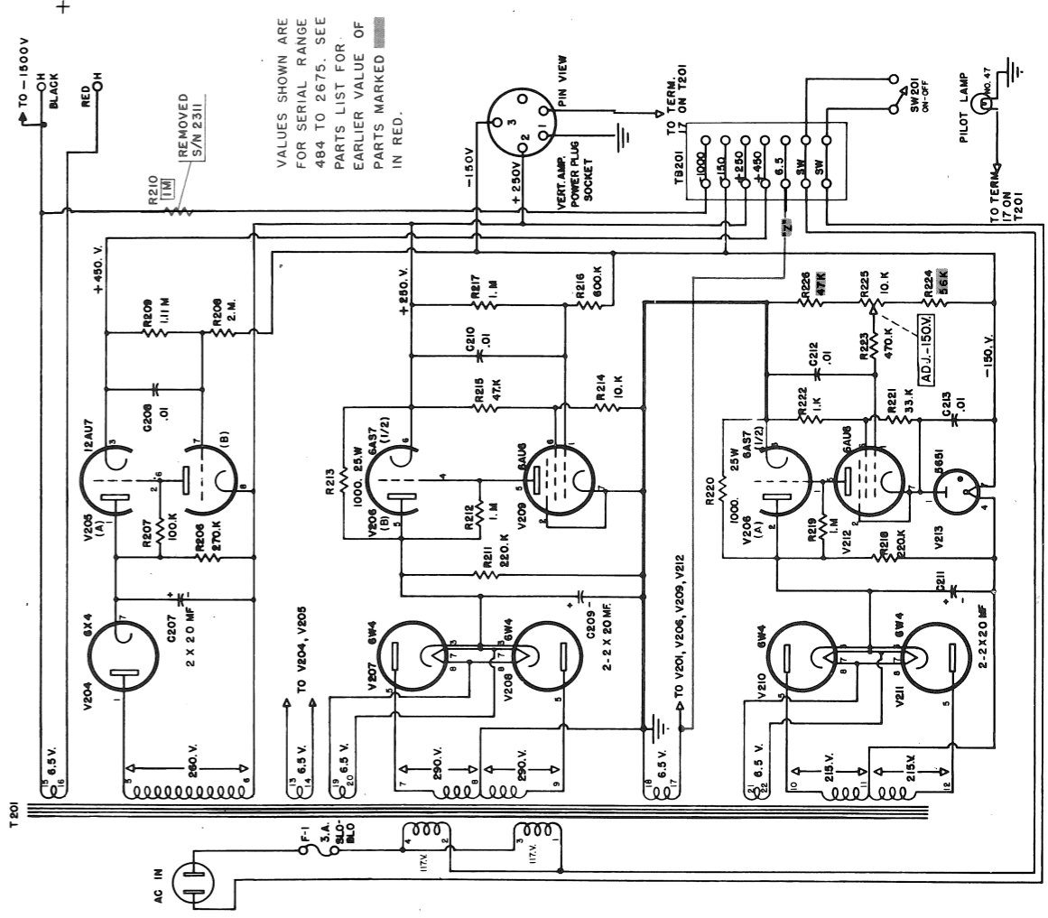
TYPE 512 OSCILLOSCOPE + POWER SUPPLY
